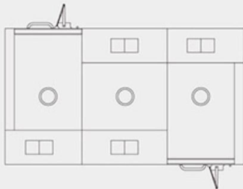
Small Z-shaped air shower tunnel
